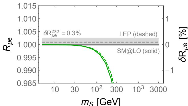
Figure 10. SM expectation for the ratio R_{\mu e} and its minimum deviation due to muon mixing if a singlet scalar model UV completed by fermion mediators resolves the (g - 2)_\mu anomaly. The gray solid line represents the leading order-calculation, and the gray dashed line with shaded band shows the experimental result from LEP with an error of 0.3% [120]. The solid (dashed) green line represents the fermion UV completion \mathcal{L}_I ( \mathcal{L}_{II} ) from eq. (C.1).
