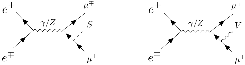
Figure 5. Representative Feynman diagrams that yield singlet scalar (left) and vector (right) production at a B -factory via e^+e^- annihilation. The BABAR and Belle II search strategies discussed in section 4 involve the 4\mu channel in which S/V \rightarrow \mu^+\mu^- decays yield 4\mu final states with an opposite-sign di-muon resonance that reconstructs the singlet’s mass.
